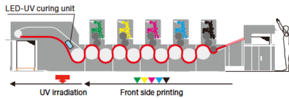
Installation example on 5-color, 1,060 mm format, straight press
